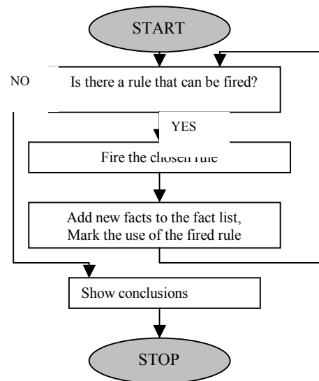
Fig. 1 The scheme of forward chaining.
